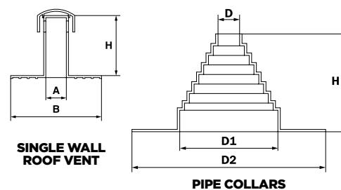
PIPE COLLARS
