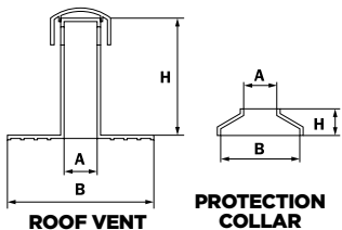
ROOF VENT
