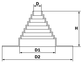
PIPE COLLARS
